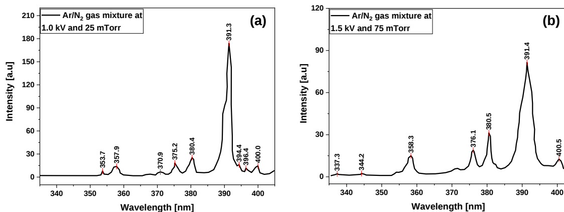
Figure 5. A scan of the optical emission spectrum of a DC hollow cathode discharge of an Ar/N 2 gas mixture was obtained at (a) applied voltage of 1 kV and pressure of 25 mTorr and (b) applied voltage of 1.5 kV and 75 mTorr.
