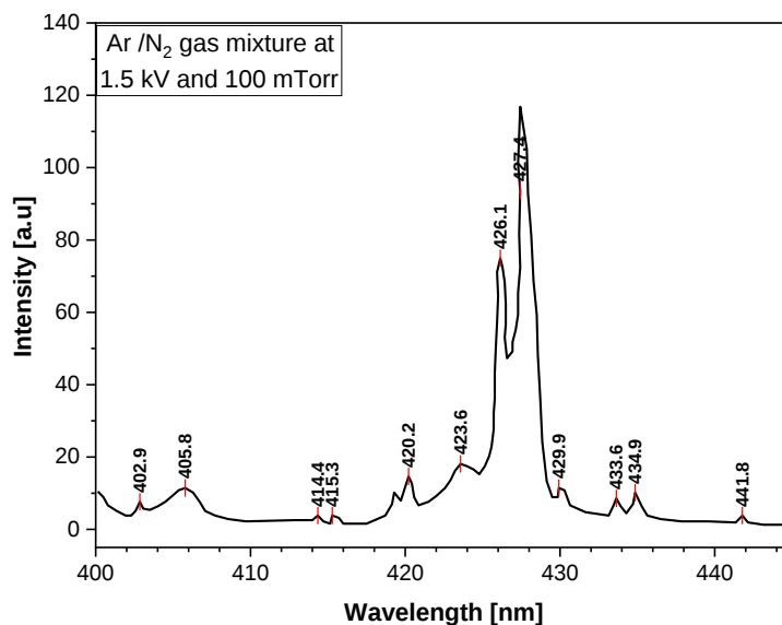
Figure 2. A scan of the optical emission spectrum of a DC hollow cathode discharge of Ar/N 2 gas mixture, recorded in the wavelength range of 400 nm to 445 nm, was obtained at a gas pressure of 100 mTorr and an applied voltage of 1.5kV.
