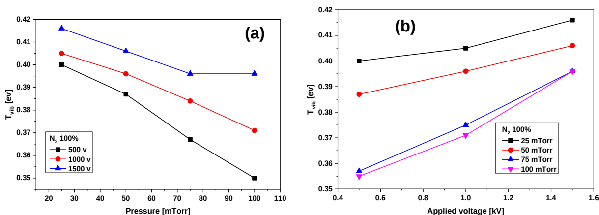
Figure 7. The plot of T_{\text{vib}} of N 2 as a function of (a) gas pressure at various applied voltages, 0.5, 1, and 1.5 kV, and (b) at various gas pressures, 25, 50, 75, and 100 mTorr.
